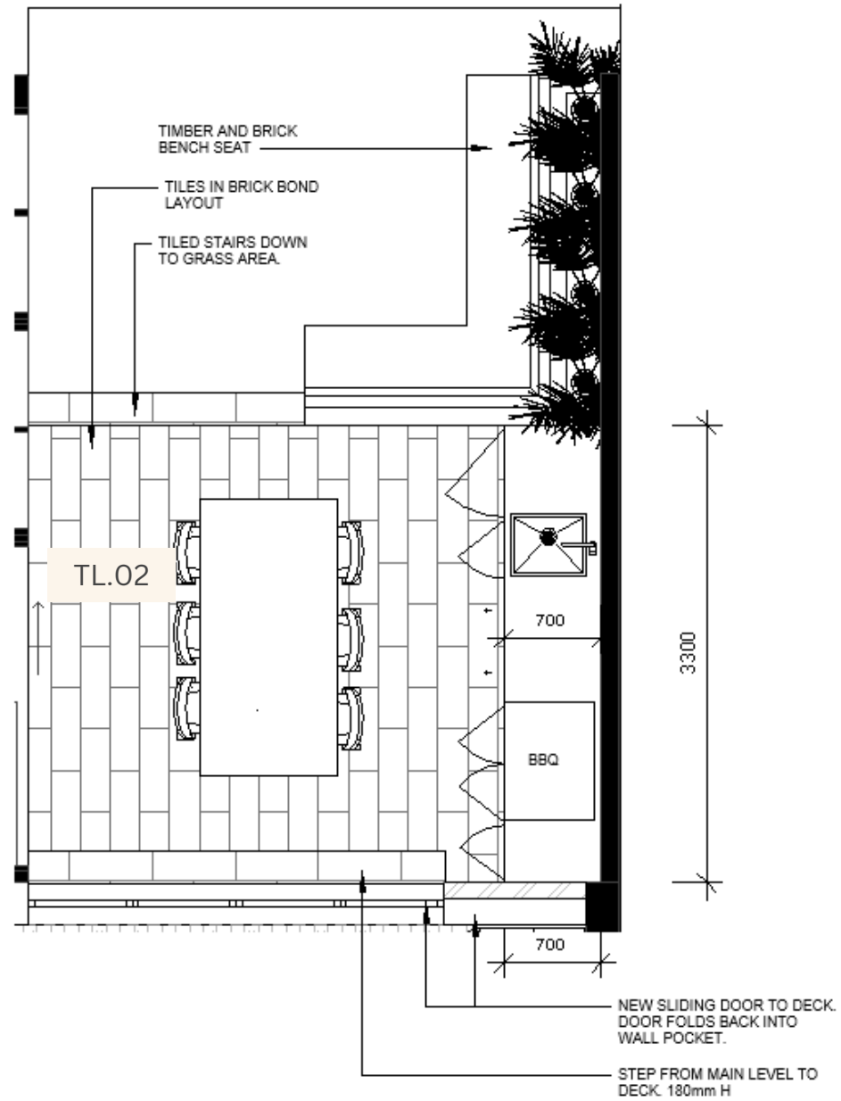
PLAN VIEW
